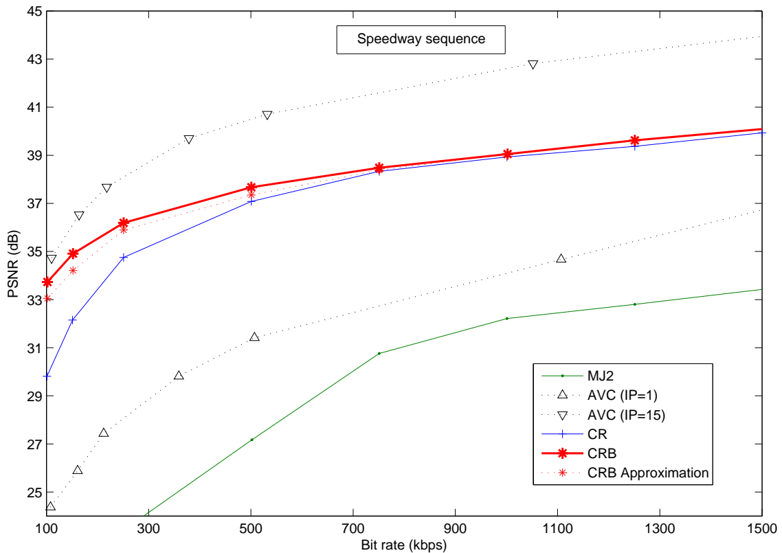
Fig. 7. Rate distortion curves of the proposed algorithms compared with MJ2 and AVC for the Speedway sequence. Frame rates and encoding parameters are defined in the text.
