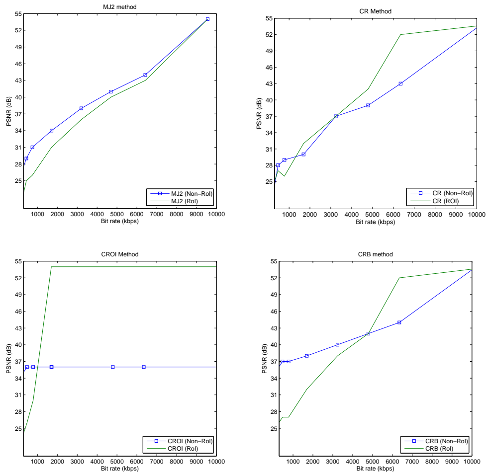
Fig. 10. RoI and non-RoI quality as a function of the total transmission rate for the CR, CROI, CRB and MJ2 methods ( Speedway sequence).
