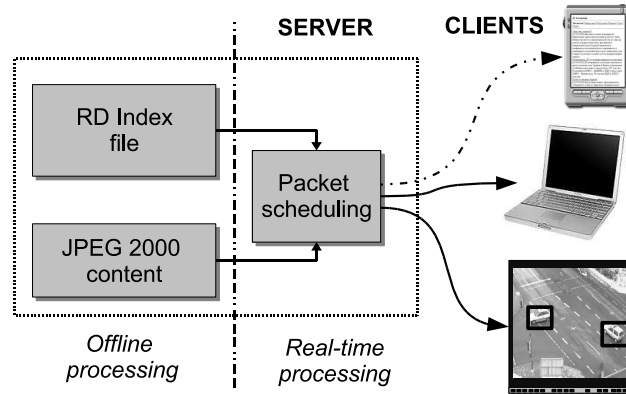
Fig. 1. Proposed video server architecture. Using a pre-calculated index, the server selects the optimal packets to transmit to each client, based on their individual needs and resources. Three types of clients are illustrated: a PDA client with a low resolution and low bandwidth, a laptop client with a high bandwidth and a client focusing on two regions of interest for which he is expecting a high quality.
