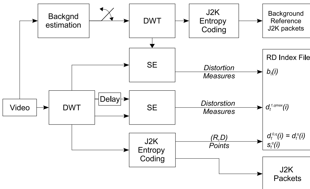
Fig. 3. Off-line operations leading to the creation of the RD index file at the server.
