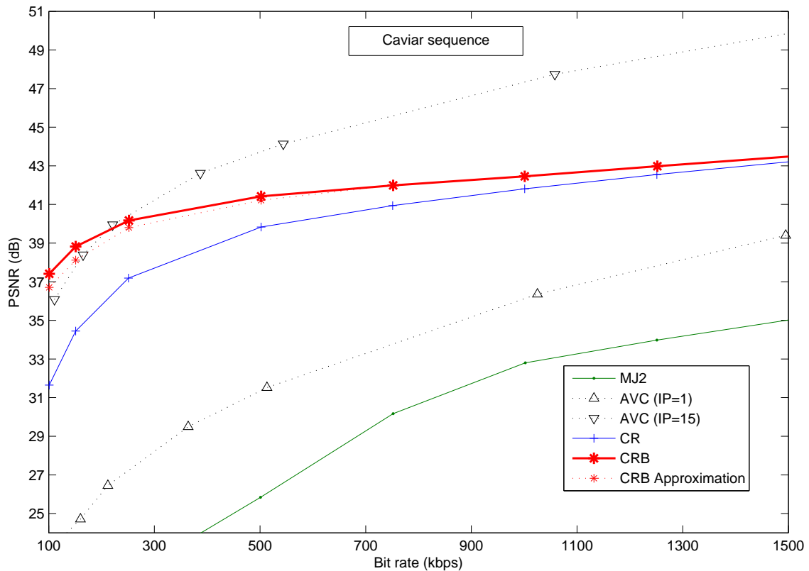
Fig. 8. Rate distortion curves of the proposed algorithms compared with MJ2 and AVC for the Caviar sequence. Frame rates and encoding parameters are defined in the text.
