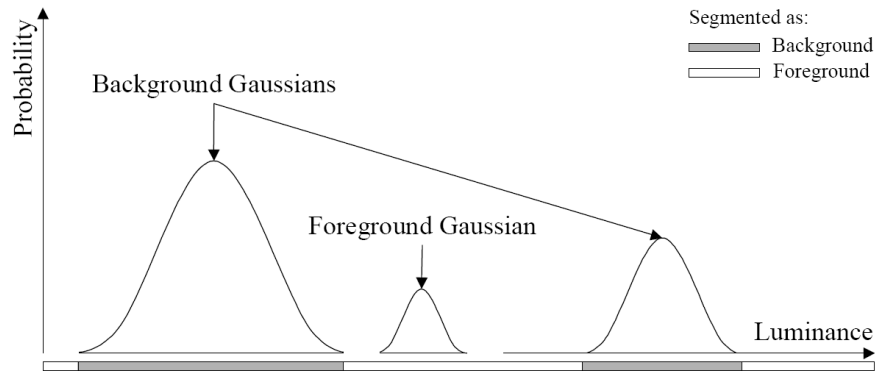
Fig. 6. Statistical modeling of a background pixel using three Gaussians. Multiple Gaussians aggregate the pixel luminance values observed in a sliding window.
