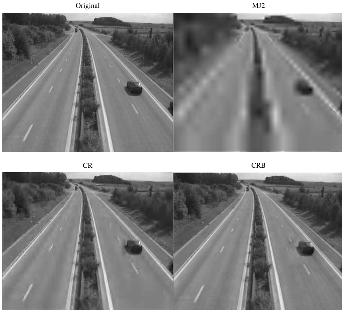
Fig. 9. MJ2, CR, and CRB methods for the 10th frame of the Speedway sequence transmitted at 250 kbps, 25 fps and in CIF format.
