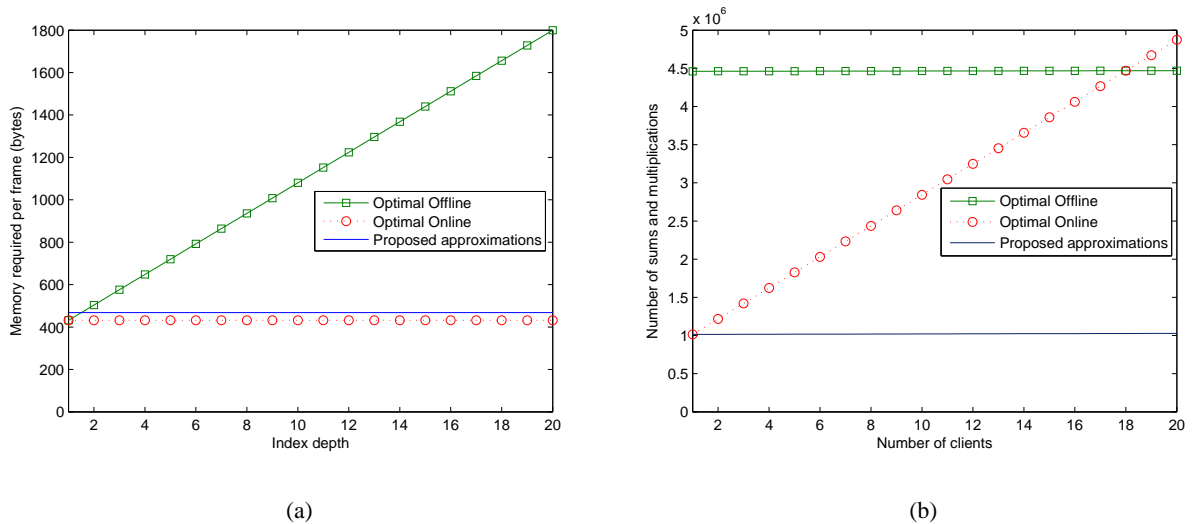
Fig. 5. Comparison of (a) memory and (b) computational resources for three different implementations of the proposed replenishment framework. Memory is depicted as a function of the index depth I_d , while computational resources are presented as a function of the number of server clients.
