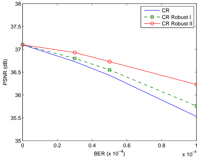
Fig. 12. Comparison of three replenishment methods as a function of the channel bit error rate for the Speedway sequence at 500 kbps. Transmitted JPEG 2000 packet are considered as lost as soon as one of their bits becomes erroneous. The three methods are described in the text.
