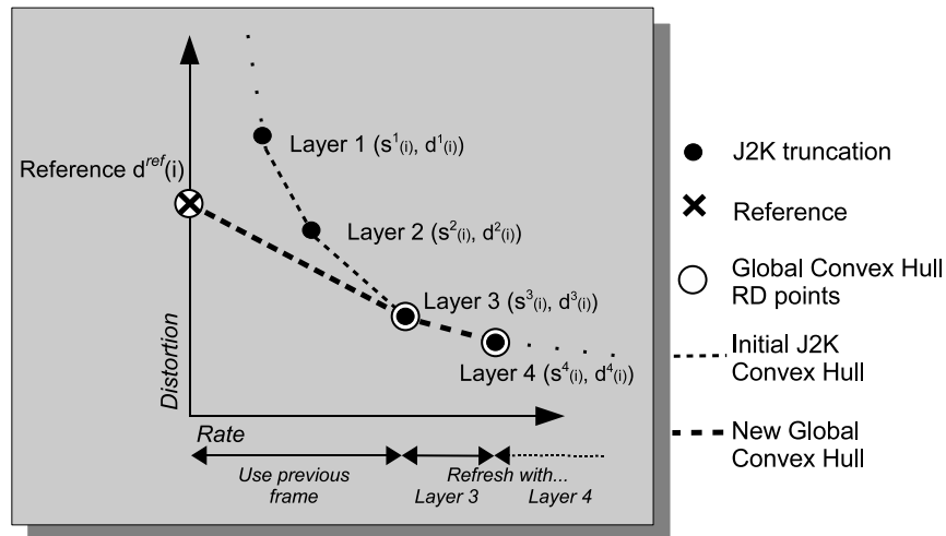
Fig. 2. Rate-Distortion points for a given precinct. The figure presents both the set of RD points corresponding to the JPEG 2000 codestream truncation points ( dots ), and the additional RD point corresponding to the approximation of the precinct by the reference image ( cross ). The set of RD trade-offs provided by the JPEG 2000 codestream lie on a convex-hull. The novel trade-off authorized by the reference image lie on the distortion axis ( R = 0 ). Global convex-hull (circles) has to be considered for RD optimal allocation at image level.
