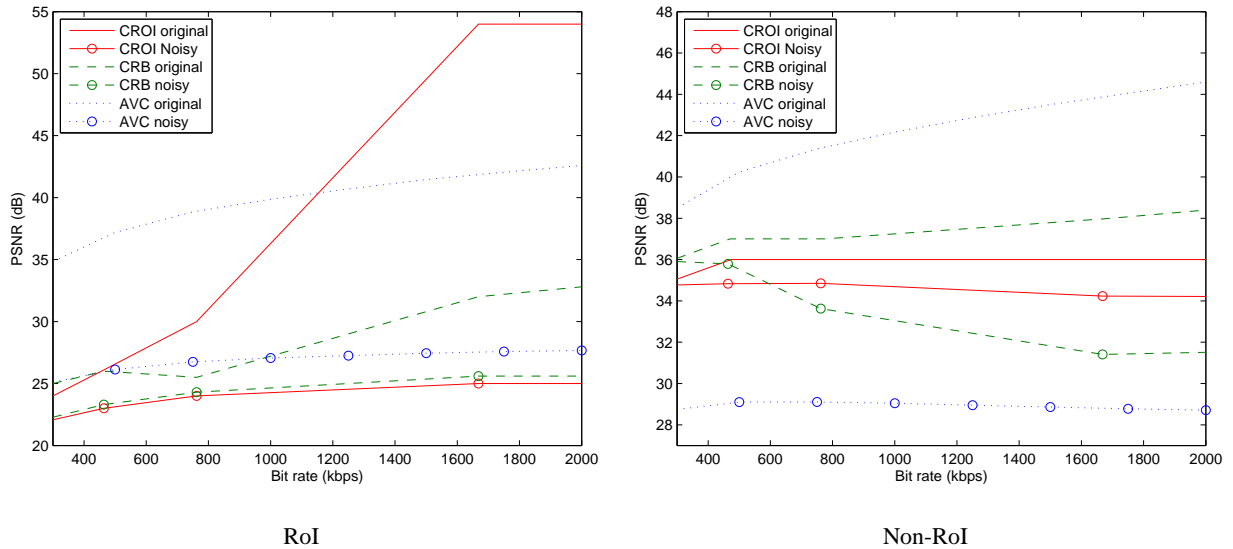
Fig. 11. RoI and non-RoI quality for the CROI, CRB, and AVC methods in normal and noisy conditions ( Speedway sequence). In all cases, the PSNR is calculated using the original (non noisy) sequence as reference.
